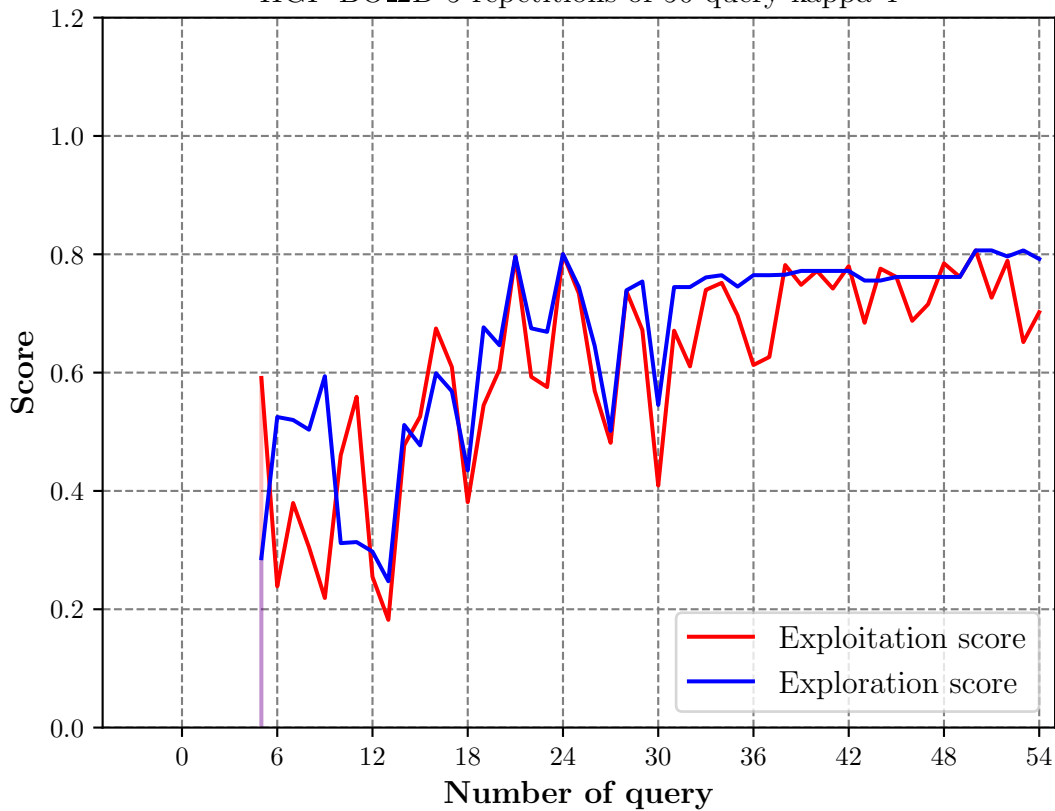
HGP-BO_2D 5 repetitions of 50 query kappa 4
